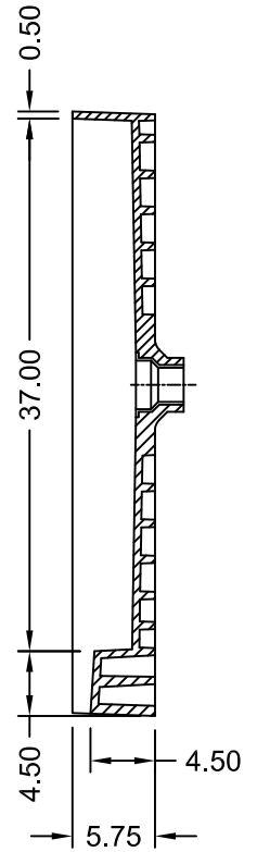
SECTION B-B
